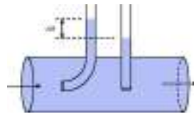
Pitot Tube HAN/HVHL
